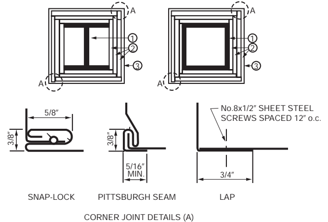
FIGURE 722.5.1(2) GYPSON-PROTECTED STRUCTURAL STEEL COLUMNS WITH SHEET STEEL COLUMN COVERS
