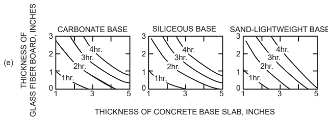
FIGURE 722.2.2.3(2) FIRE-RESISTANCE RATINGS FOR CONCRETE ROOF ASSEMBLIES
